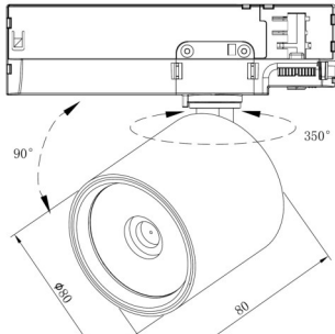
DIMENSIONS: Ø80 x 80 mm
